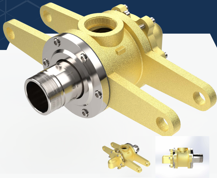
Rotary Joint for steam
