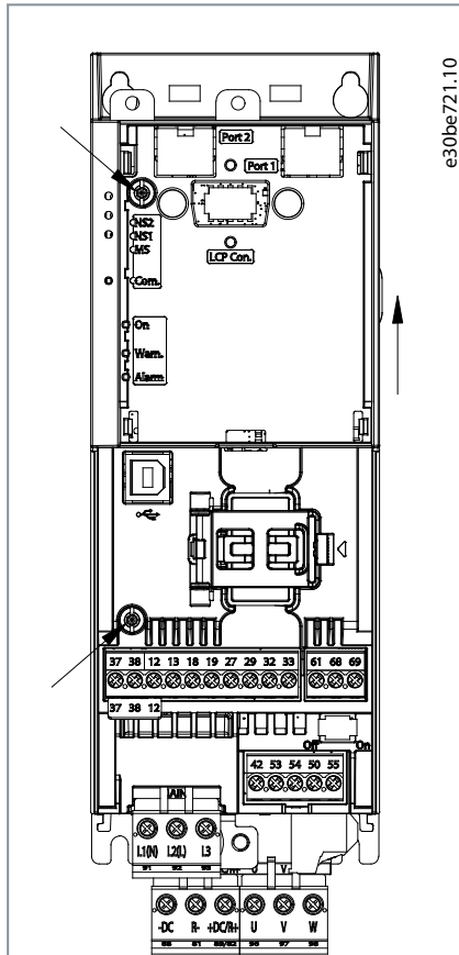
Illustration 3: Loosen the Old Control Card Cassette
