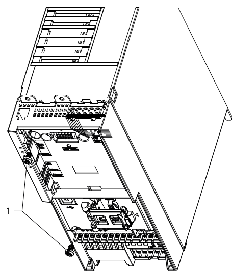
Illustration 6: Tighten Screws
