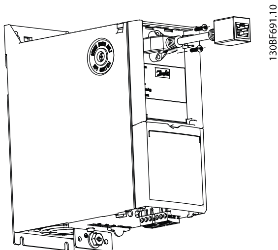
Illustration 1.1 Mounting the Male LCP 21-RJ45 Converter Plug
